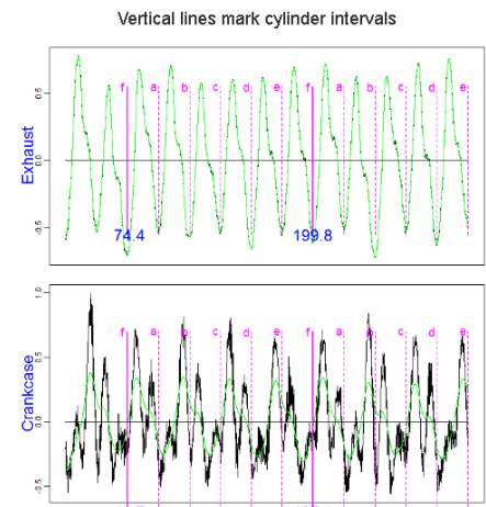
Figure 8: The Polygraph Model of the Pressure vs. vibration in the EP Signature for the subject engine.
