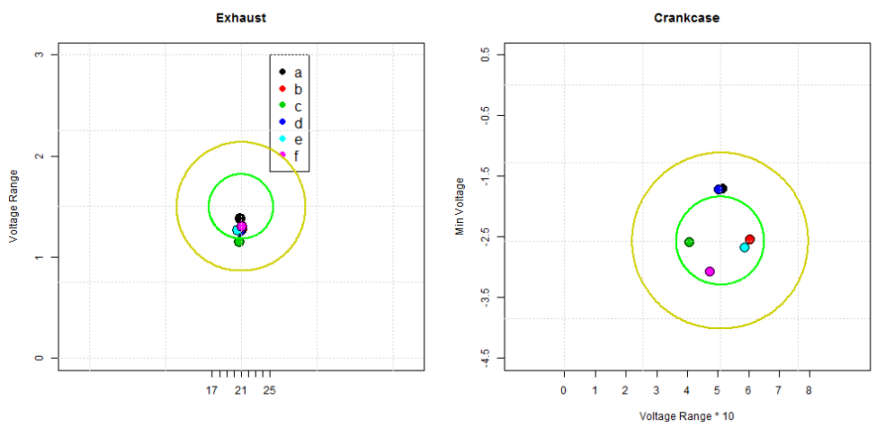
Figure 5: Engine Integrity diagram showing the (dis)similarity of the value of parameters for each cylinder derived from the Signature data.
